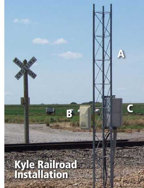
A–Tower, B–Antenna, C–Railert ATR Control Box
